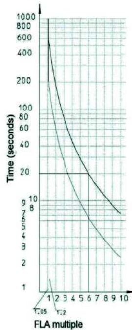
Trip class 20
