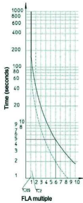
Trip class 20
