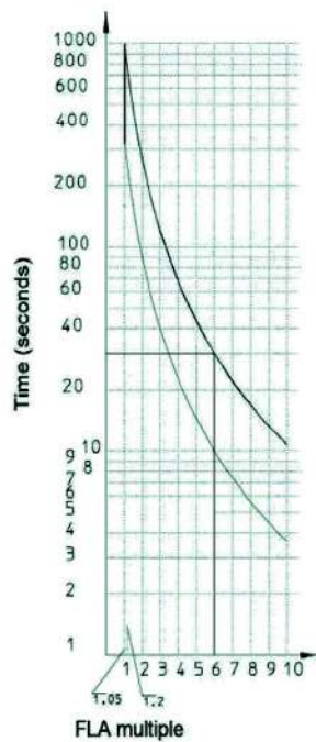
Trip class 30
