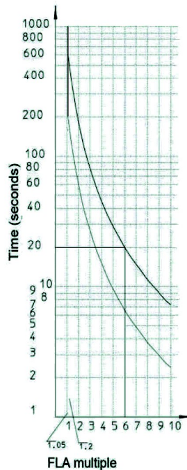
Trip class 20
