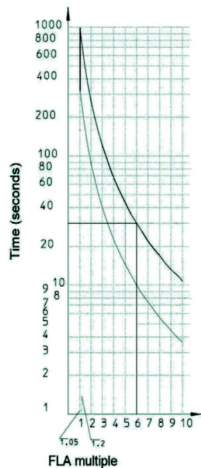
Trip class 30
