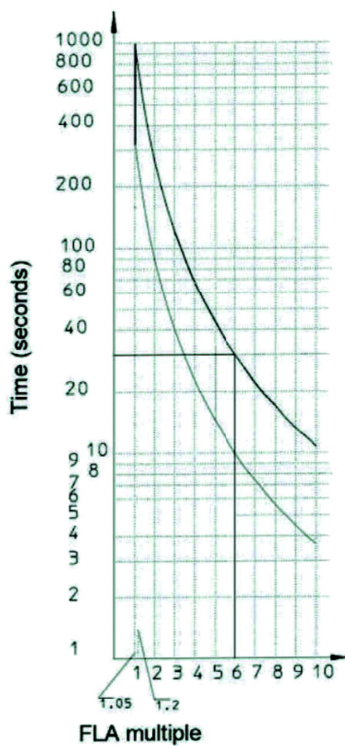
Trip class 30
